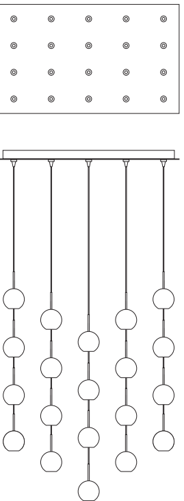
CPEJRT20(FINISH)1831(HAL, LED) EZ JACK 20 Lite Canopy FINISH PN, SN LAMP HAL, LED DIMENSIONS 18" x 31" Rectangular
