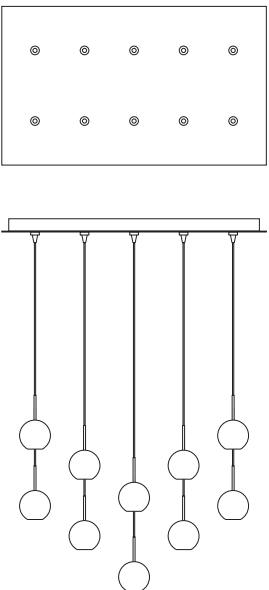
CPEJRT10(FINISH)1831(HAL, LED) EZ JACK 10 Lite Canopy FINISH PN, SN LAMP HAL, LED DIMENSIONS 18" x 31" Rectangular
