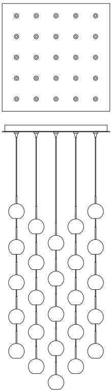
CPEJSQ25(FINISH)(HAL, LED) EZ JACK 25 Lite Canopy FINISH BZ, PC, PN, SN, WH LAMP HAL, LED DIMENSIONS 24" Square
