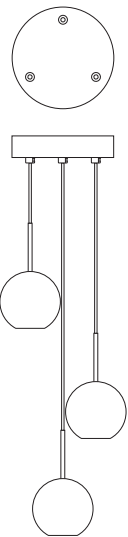
CPSRRN3(FINISH)(HAL, LED) STRAIN RELIEF 3 Lite Canopy FINISH BZ, PN, SN LAMP HAL, LED DIMENSIONS 7.5" Round
