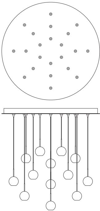
CPEJRN22(FINISH)36(HAL, LED) EZ JACK 22 Lite Canopy FINISH PN, SN LAMP HAL, LED DIMENSIONS 36" Round
