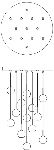
CPEJRN13(FINISH)24(HAL, LED) EZ JACK 13 Lite Canopy FINISH PN, SN LAMP HAL, LED DIMENSIONS 24" Round
